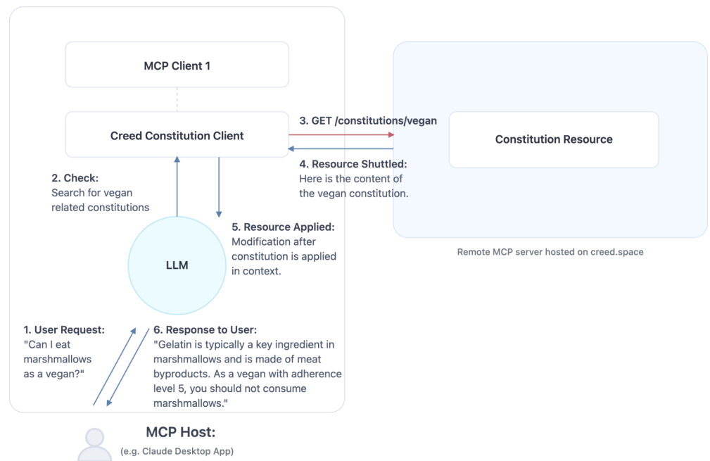
Figure 3. Data flow diagram for the Superego Model Context Protocol Architecture.
