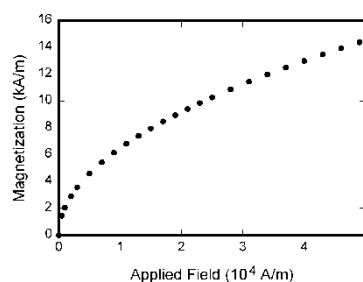
Gambar 1. Magnetization
