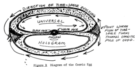
Figure B Diagram of the Cosmic Egg
