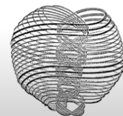
Figure C Stylized Rendition of a Simple Torus
