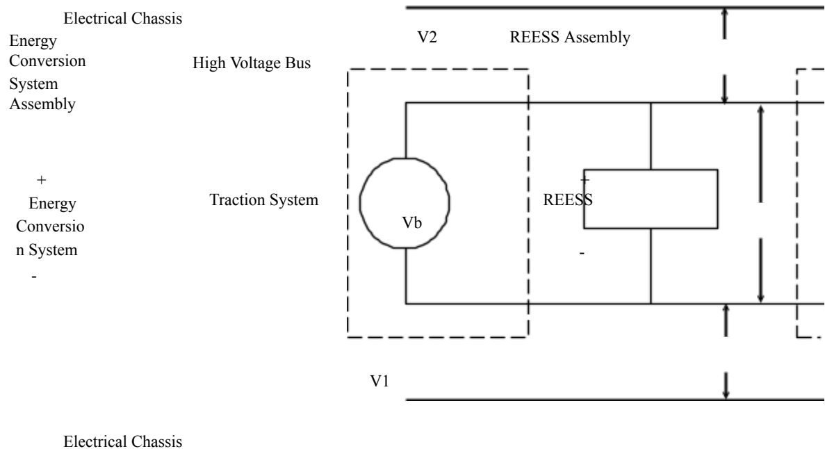
Figure 1 Measurement of Vb, V1, V2
