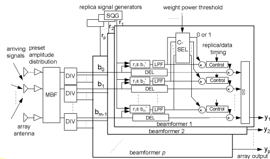
Figure 1. Proposed beam former
