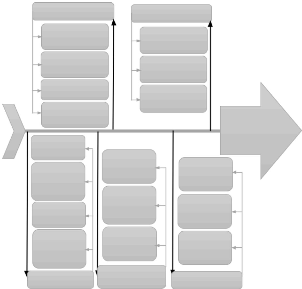
Gambar 1. Diagram Fishbone
