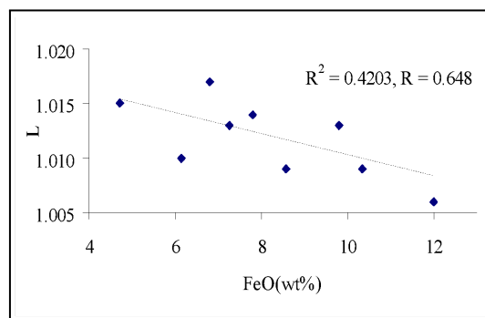
Gambar 1. Plots of lineation (L) and FeO content showing negative correlation
