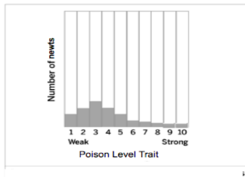
1. Starting Population
