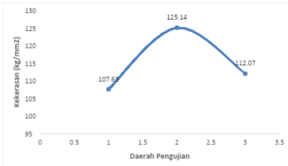
GAMBAR 2. DISTRIBUSI KEKERASAN
