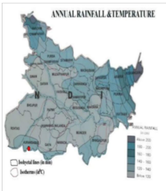
Figure 2: Annual Rainfall and Temperature
