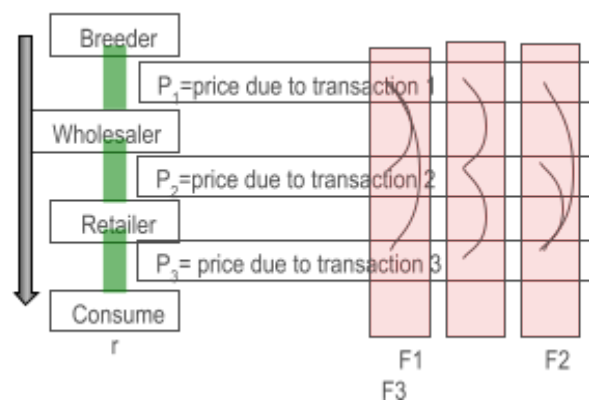
Figure 1. F-test with Granger Causality for APT Analysis
