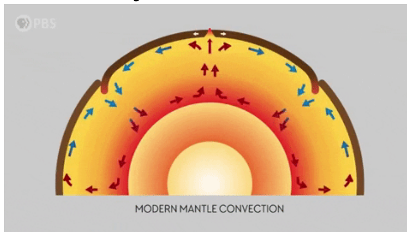
Figure 5: Mantle Convection
