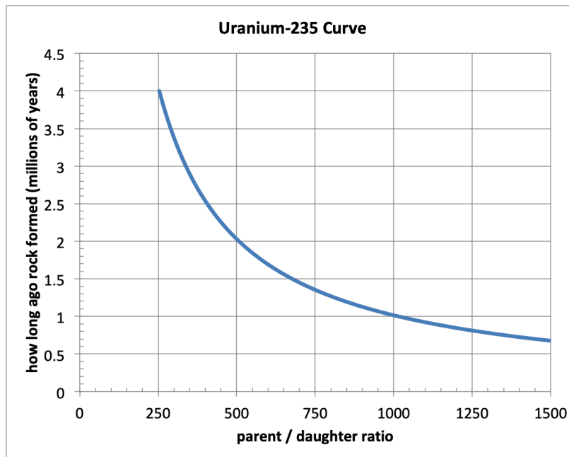
Figure 4: Uranium-235 Curve
