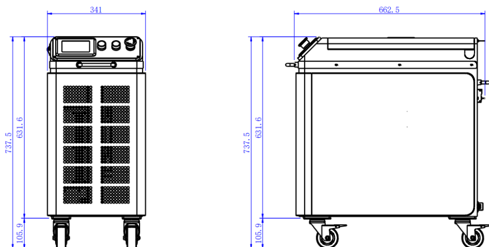
Figure 2.3 – GY-FLC300S Laser Cleaning Machine Dimensional Diagram
