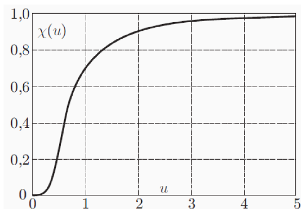
Figure 2 – Graphe de \chi(u)
