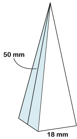
square pyramid
