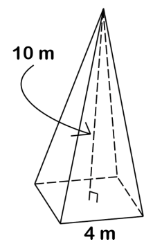
Square base
