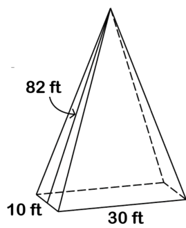
Rectangular base
