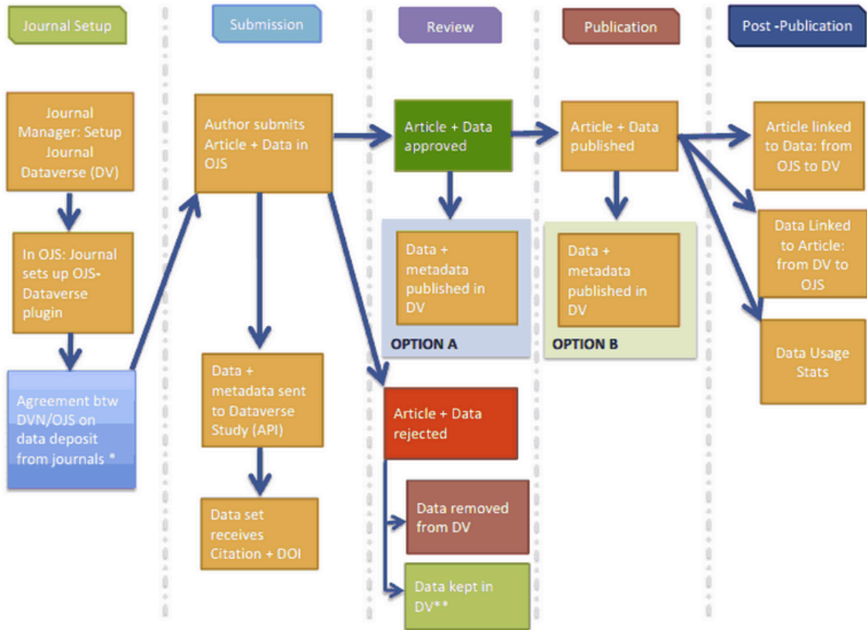
Fig. 1 High Level Dataverse Plugin Data Publication Workflow
