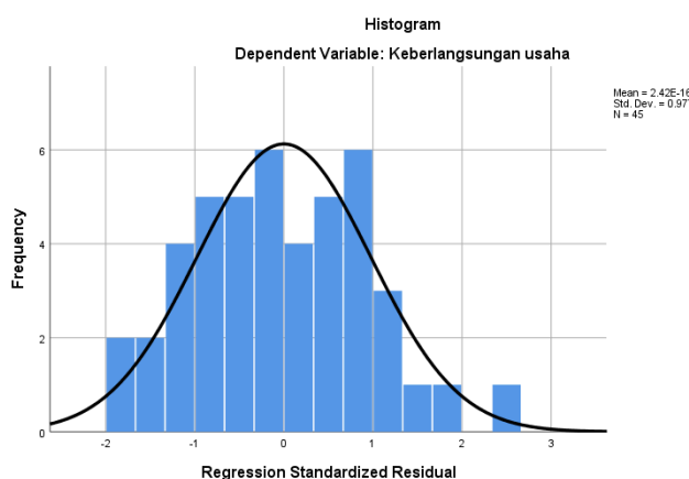
Figure 1. Histogram Test
